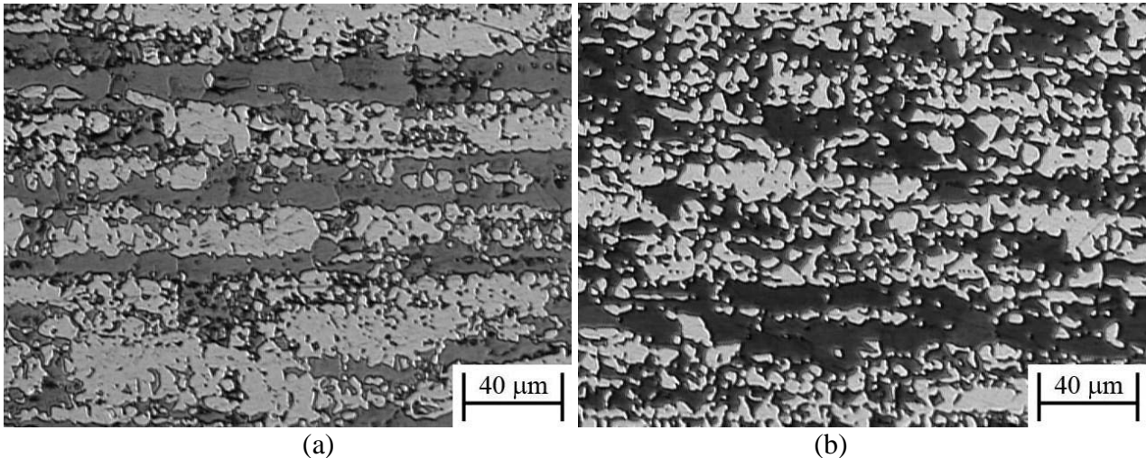
Figure 1: Microstructures of UNS S32304 (a) and UNS S32205 (b) steels in the as received condition.
