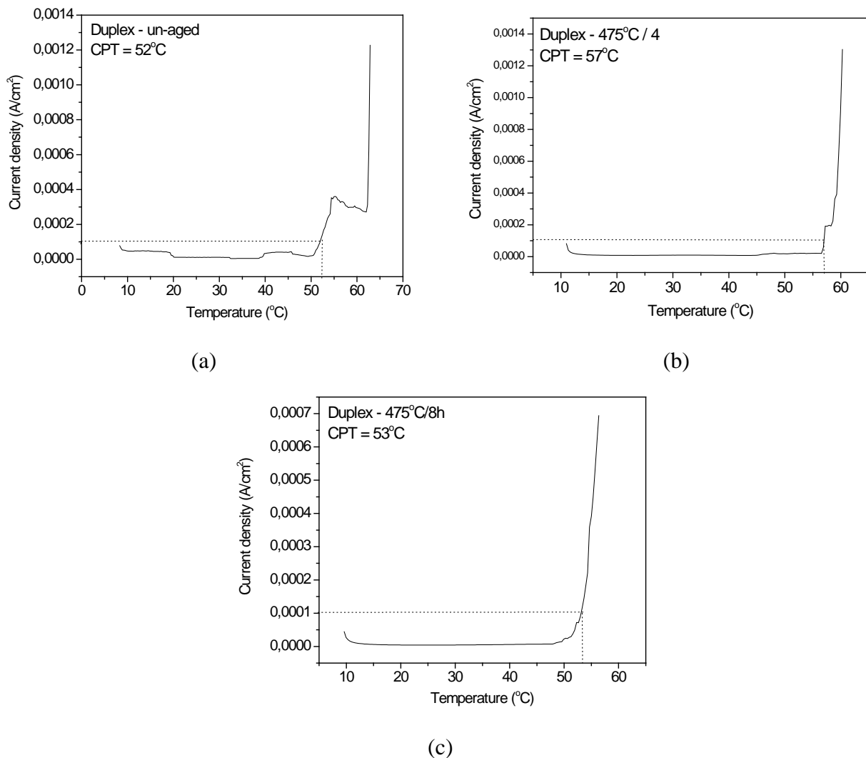
Figure 7: Density current x temperature curves for E = 0.700V_{SCE} for determination of CPT in duplex UNS S32205: (a) Annealed; (b) Treated at 475^{\circ}C for 4 hours (c) Treated 475^{\circ}C for 8 hours.
