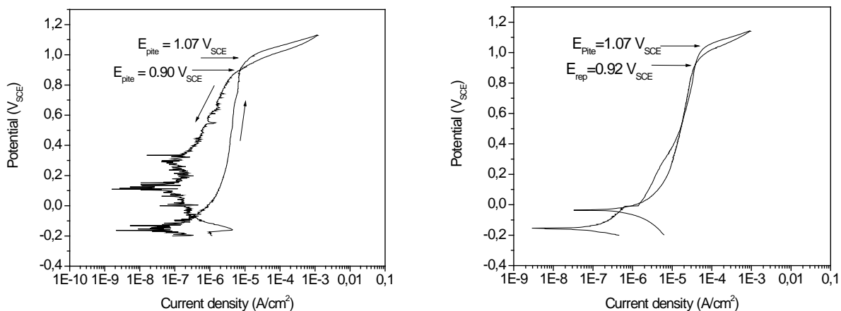
Figure 6: Cyclic polarization curves for duplex UNS S32205: (a) Annealed; (b) Treated at 475°C for 4 hours.
