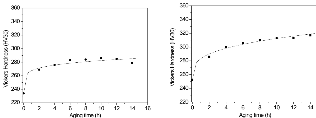
Figure 5: Curves fitted with equation (1) and parameters of table 2: (a) lean duplex; (b) duplex.
