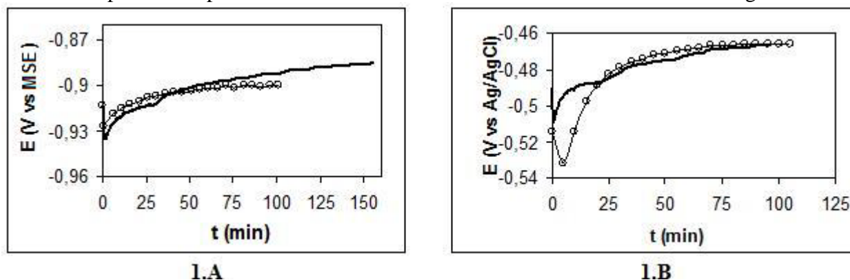
Figure 1: Open circuit potential curves of 430 SS, in absence ( \circ ) and in the presence of azoles in 1 \times 10^{-3} \text{ mol L}^{-1} (—) concentration in media: (1.A) 1 \text{ mol L}^{-1} \text{ H}_2\text{SO}_4 ; and (1.B) 1 \text{ mol L}^{-1} \text{ HCl} .
