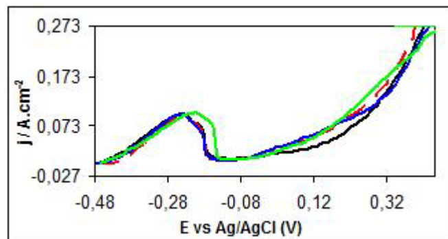
Figure 3 - Potentiodynamic anodic polarization curves of 430 SS in HCl media in the absence (—) and presence of indole in the following concentrations (—) 1 \times 10^{-3} , (—) 5 \times 10^{-4} e (—) 1 \times 10^{-4} \text{ mol.L}^{-1} .
