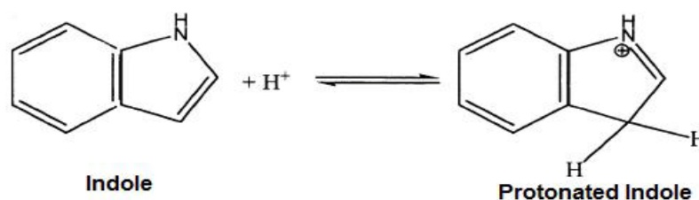
Figure 7 – Mechanism proposition of protonation to Indole in media of HCl.
