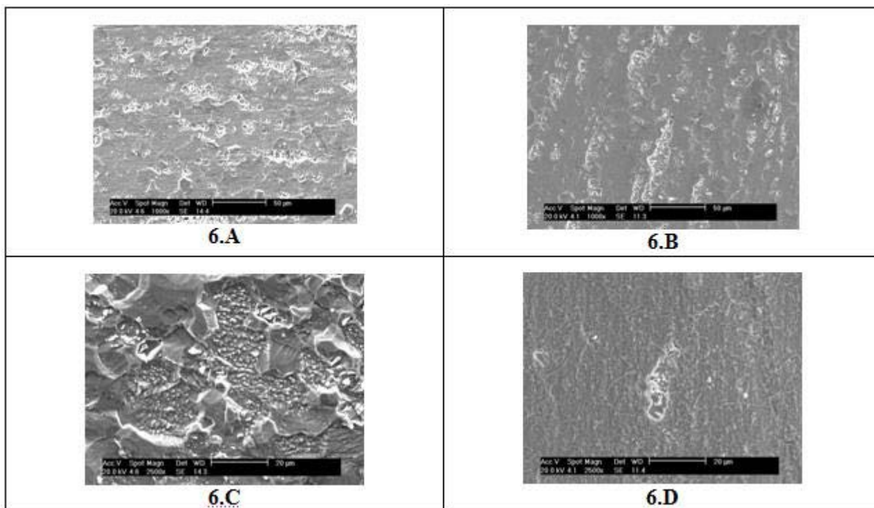
Figure 6 - Scanning Electron Microscope (SEM) of 430 stainless steel ABNT in: (A) 1 \text{ mol L}^{-1} \text{H}_2\text{SO}_4 in the absence of indole, (B) 1 \text{ mol L}^{-1} \text{H}_2\text{SO}_4 in the presence of indole, (C) 1 \text{ mol L}^{-1} \text{HCl} in the absence of indole and (D) 1 \text{ mol L}^{-1} \text{HCl} in the presence of indole.
