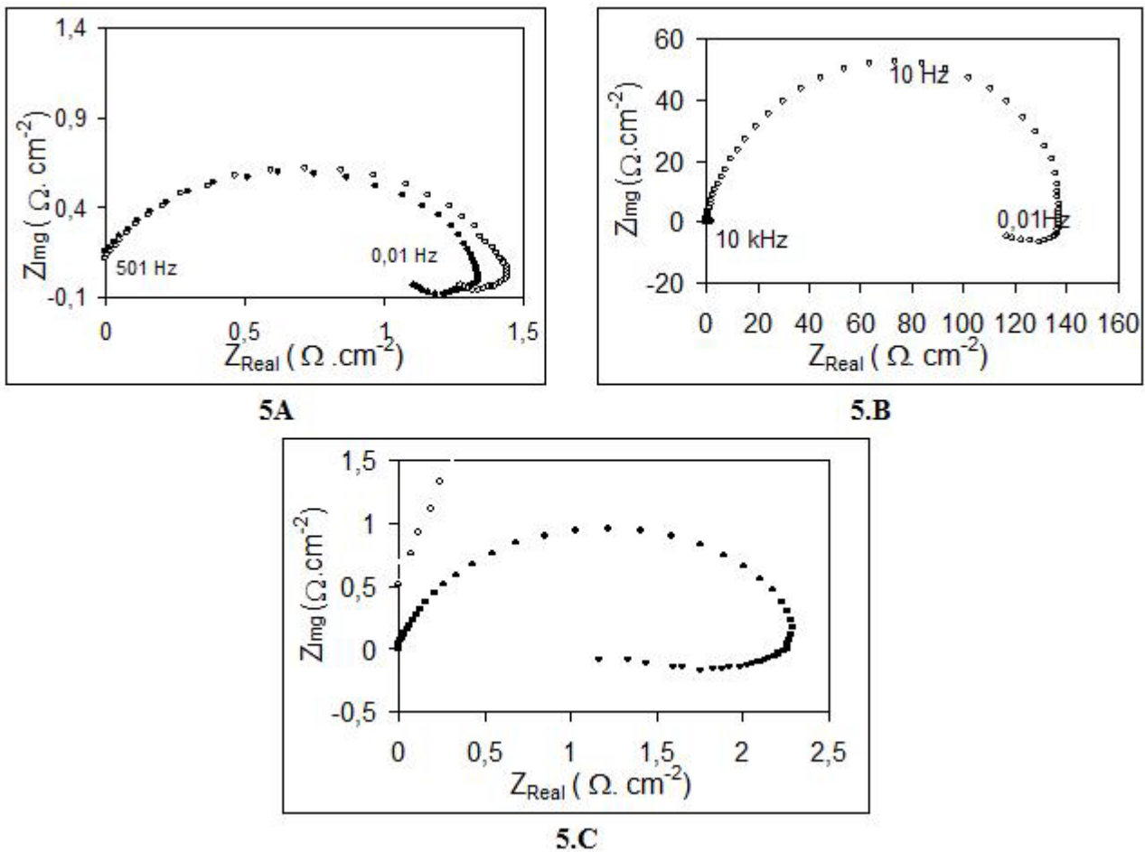
Figure 5: EIS Diagram for 430 SS in (5.A) 1 mol L -1 H 2 SO 4 and (5.B) 1 mol L -1 HCl in the absence (●) and presence (◊) of indole at a 1x10 -3 mol L -1 concentration. EIS carried out in E corr and E perturbation = ± 10 mV vs. MSE. In (5.C) the expansion of (5.B) is shown for better visualization of the curve in the absence of Indoles in 1 mol L -1 HCl.
