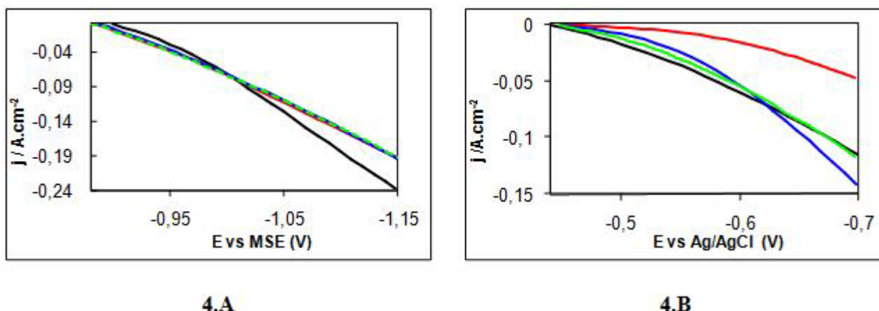
Figure 4: Cathodic potentiodynamic polarization curves of 430 SS in the (4.A) H 2 SO 4 and (4.B) HCl media in the absence (—) and presence of Indole in the following concentrations: (—) 1x10 -3 , (—) 5x10 -4 e (—) 1x10 -4 mol L -1 .
