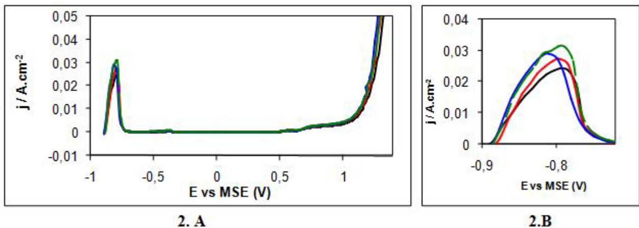
Figure 2 - Potentiodynamic anodic polarization curves of 430 stainless steel in 1 \text{ mol L}^{-1} \text{H}_2\text{SO}_4 media in the absence (—) and presence of indole concentrations (—) 1 \times 10^{-3} , (—) 5 \times 10^{-4} and (—) 1 \times 10^{-4} \text{ mol L}^{-1} in the following regions: (2.A) active-passive-transpassive and (2.B) active.
